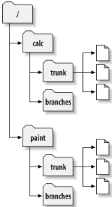
Figure 4.2. Starting repository layout
