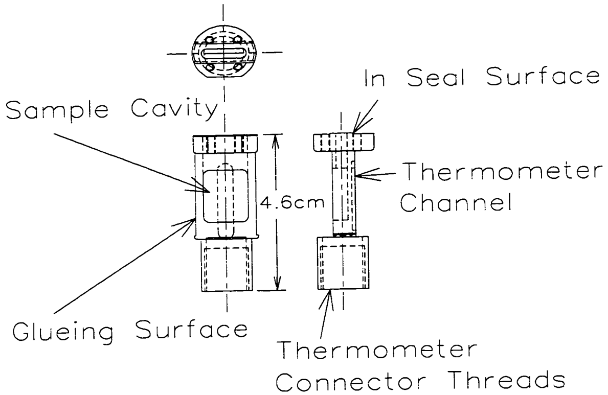
Figure B.1: A scale drawing of the (Ag) powder cell used in the dilution refrigerator. The sample is loaded via the slot in the top of the cell which is surrounded by the 4-hole pattern of threaded holes for the sealing screws. Note the relieved area for the indium seal. The seal is made with a plug (not shown) also made of 99.9% Ag.
