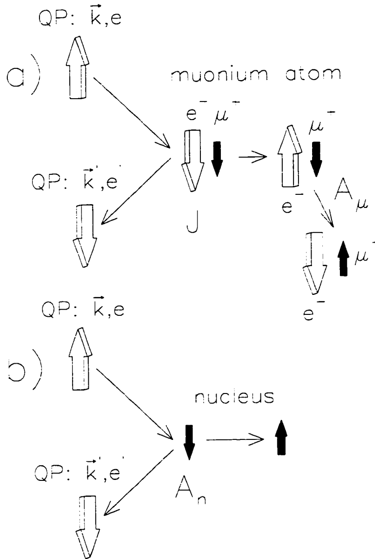
Figure 3.10: In each case a quasiparticle (QP) at the Fermi Surface with initial momentum \mathbf{k} and energy \epsilon scatters magnetically from the local moment. a) Spin exchange of a muonium atom (with subsequent evolution due to the muon-electron hyperfine interaction A_\mu ) vs. b) Electron-Nuclear spin-flip. In the spin exchange with the paramagnetic muonium, the electron Zeeman energies cancel; whereas in the latter, the nuclear and electron Zeeman energies do not.
