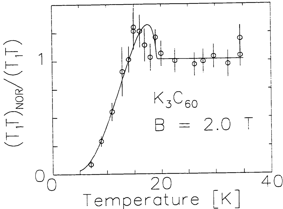
Figure 4.23: Temperature dependence of the spin relaxation rate of \text{Mu}@C_{60} in \text{K}_3\text{C}_{60} at a field of 2.0 T. The fit is to the Hebel-Slichter integral Eq. (3.9) with a broadened DOS of the form Eq. (3.12).
