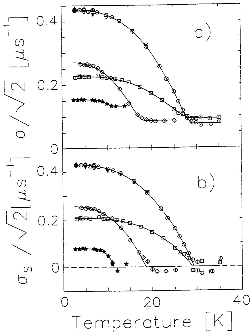
Figure 4.19: a) Second moments of the \mu SR lineshape as a function of temperature in stars Na_2CsC_{60} (0.01T), diamonds K_3C_{60} (1.0T), Rb_3C_{60} (circles 1.0T, triangles 0.5T, nablas 1.5T), and squares a second sample of Rb_3C_{60} (0.27T). b) Second moments corrected for the normal state values, see Table 4.5
