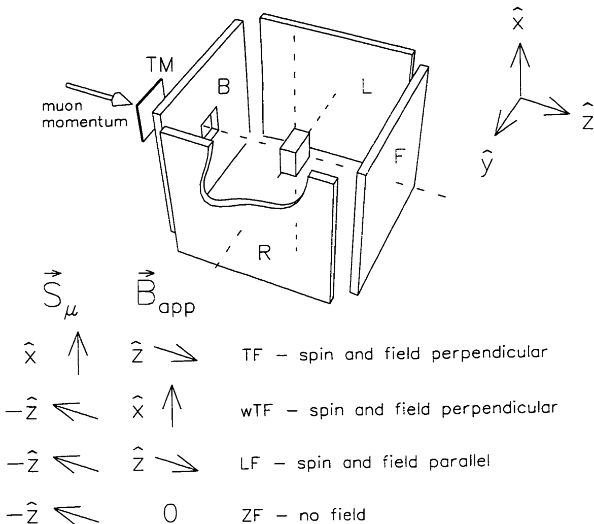
Figure 2.6: General counter arrangement for a \mu SR experiment.
