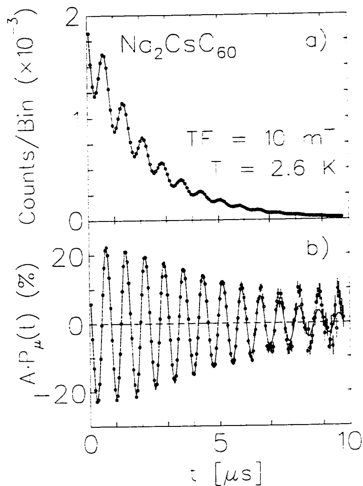
Figure 2.7: a) The time histogram of muon-positron decays detected in a single counter in \text{Na}_2\text{CsC}_{60} in 10 mT transverse field (see Eq. (2.4)). b) The same data combined with another histogram to remove the muon lifetime. A small non-relaxing signal, due to muons not stopping in the sample, is evident at late times. The relaxation is discussed in §4.2.
