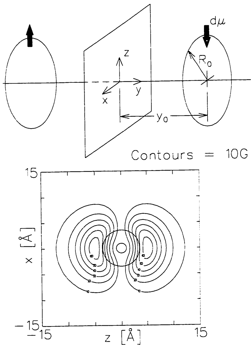
Figure 6.43: The field on a plane halfway between two (transverse) antiferromagnetically aligned moments delocalized on a ring of radius R_0 = 3.55\text{\AA} (the C_{60} radius), pictured at the top. The moments are separated by 2y_0 = 9.1\text{\AA} (the chain lattice constant). The lower panel shows the contours of the magnitude of the net field. The outermost contour is 10G, and the contour spacing is 10G. Superimposed on the contour plot are two circles representing the cross section of the equator and pole regions of the distorted C_{60} molecule (to scale). Note that there is a pronounced "hole" in the field at the y axis, and this hole is on the order of the size of the polar region of the distorted C_{60} molecule.
