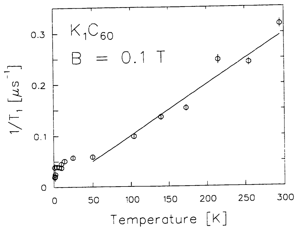
Figure 6.47: LF relaxation rate attributed to \text{Mu@C}_{60} undergoing fast spin-exchange with the conduction electrons in \text{K}_1\text{C}_{60} . The temperature dependence is not simply due to the Korringa mechanism as in \text{A}_3\text{C}_{60} . see text.
