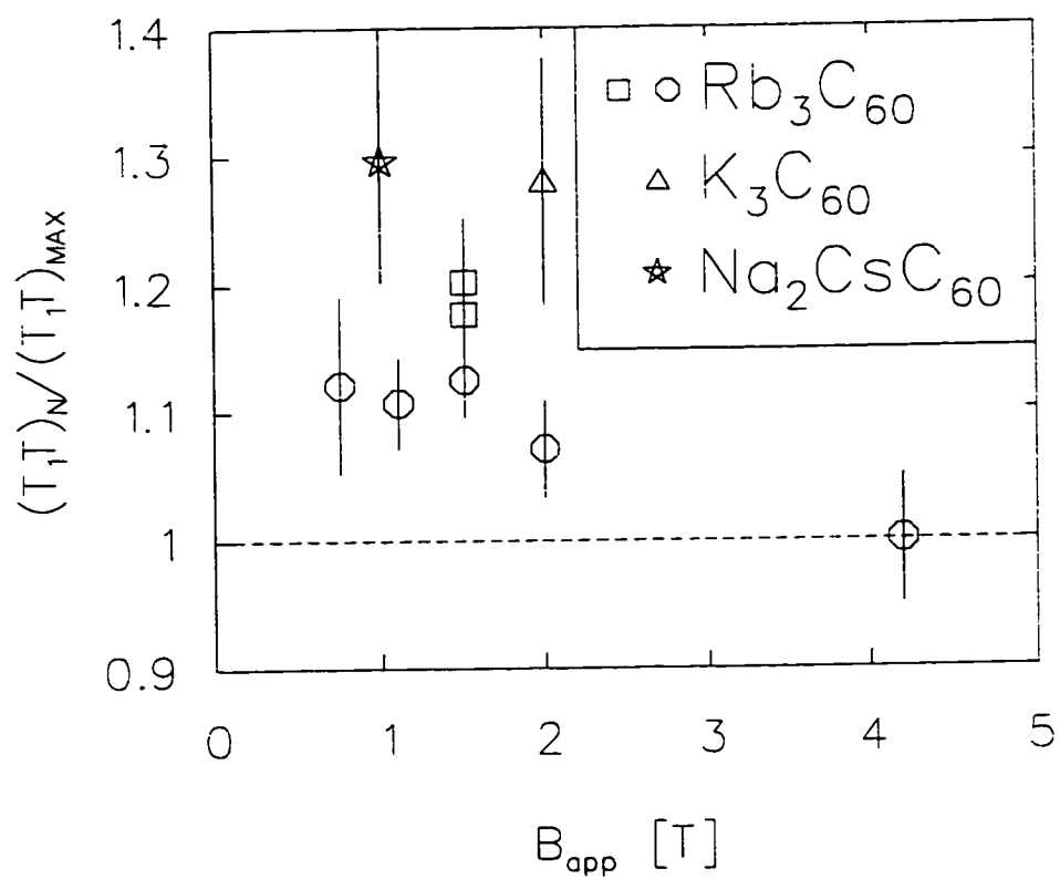
Figure 4.25: Heights of the coherence peak above the normal state as a function of field. These values were obtained from fits to a parabola near the maximum.
