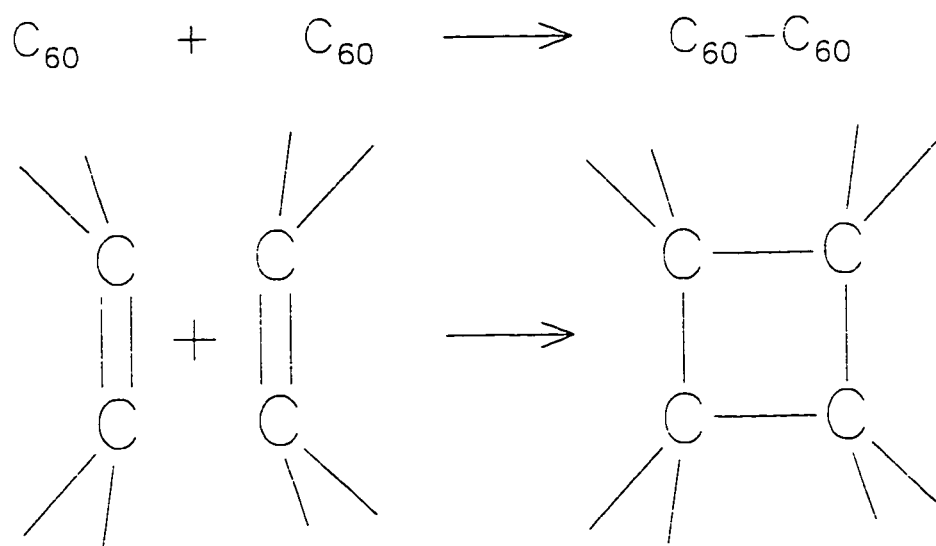
Figure 1.3: 2+2 cycloaddition bonding mechanism between two \text{C}_{60} molecules. When the double bonds of two \text{C}_{60} molecules are brought together, they break and reform into a pair of intermolecular single bonds. These intermolecular bonds are nearly sp^3 , in contrast to the intermediate nature of the hybridization for the C atoms of an isolated molecule.
