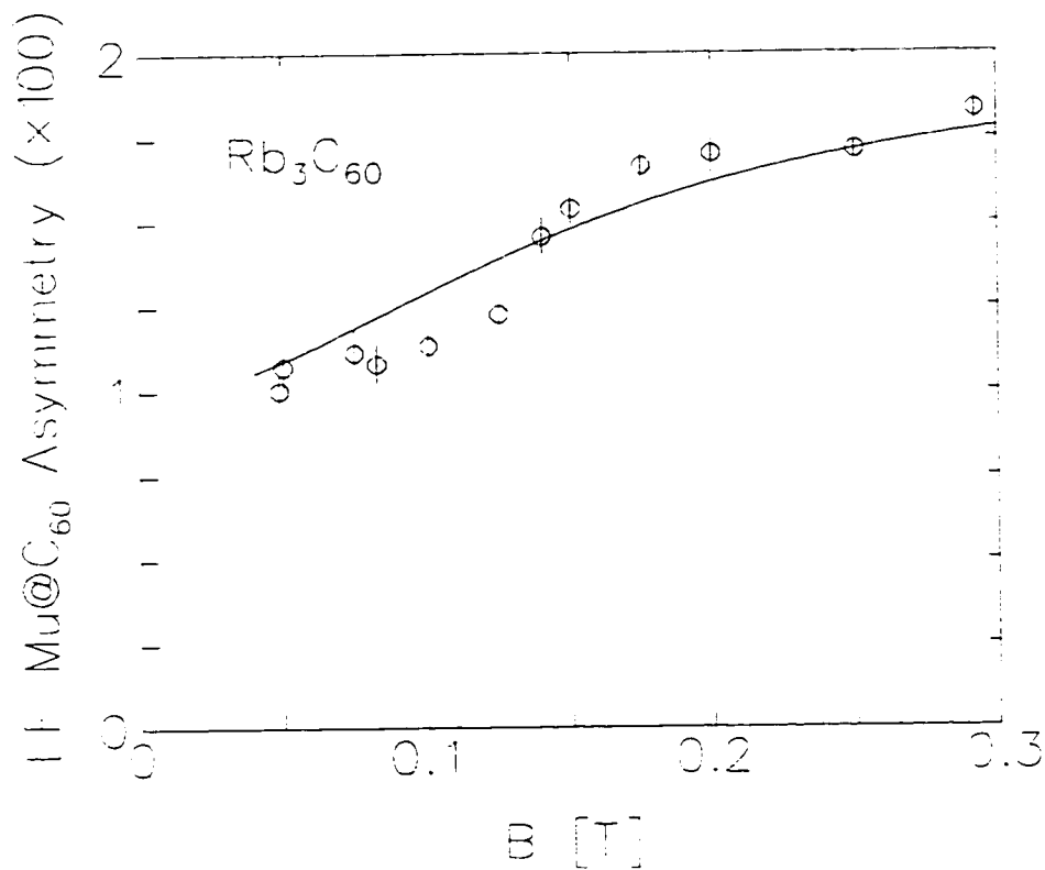
Figure 4.15: The LF dependence of the \text{Mu@C}_{60} asymmetry (decoupling curve). The field at the inflection point indicates that the \text{Mu} hyperfine parameter is large (near its vacuum value). Each point is determined from a common fit to at least 2 different temperatures, ranging from 2.5 to 15 K (e.g. Fig.4.22).
