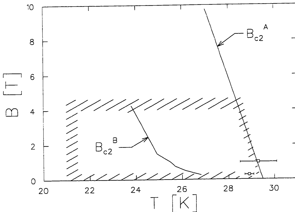
Figure 4.29: The H - T phase diagram of Rb_3C_{60} near T_c(0) \approx 29.5\text{K} . The curves are two different measurements of the upper critical field. The curve labelled A is from [31] and the curve labelled B is from [36]. The curvature of B is reminiscent of the “irreversibility line”, which separates the vortex liquid and solid phases. The hatched region is the region of the coherence peak measured by \mu\mathcal{SR} . The error bars are the measurements of T_c(H) from the TF \mu\mathcal{SR} (see Table 4.5) which are near curve A. Notice that the entire region of this diagram is contained in the extreme lower right corner of the generic phase diagram shown in Figure 3.12, so that the absence of the coherence peak expected in region (i) of Fig. 3.12 does not explain the observed damping which occurs at H/H_{c2}(0) \approx 0.1 .
