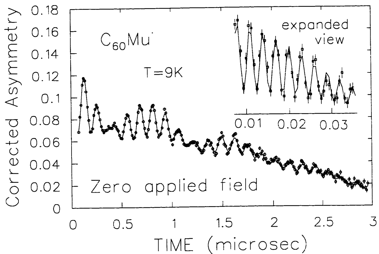
Figure 5.34: Oscillations in zero field due to anisotropy of the hyperfine interaction of the molecular radical C 60 Mu (from [172]).
