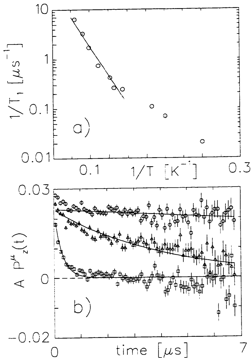
Figure 4.27: Residual relaxation at low temperature in \text{Rb}_3\text{C}_{60} . At low temperature, the relaxation deviates from the Arrhenius dependence. This behaviour is connected with either region "O" or "2C" of Fig. 3.12. The lack of field dependence and other evidence suggests that this residual relaxation may originate in crystalline disorder (rather than the vortex cores), i.e. region "O" and not "2C".
