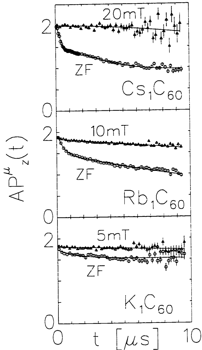
Figure 6.35: The ZF relaxation at low T in all three A_1\text{C}_{60} systems, and the quenching of that relaxation by small LF. The quenching indicates that the relaxation is due to a static magnetic field distribution in all three cases. However, the origin of the relaxation is different: for A = \text{Rb}, \text{Cs} the relaxation is due to diamagnetic muons experiencing the static fields of the low temperature magnetic phase. For A = \text{K} , the relaxation is similar, but it is nearly independent of temperature.
