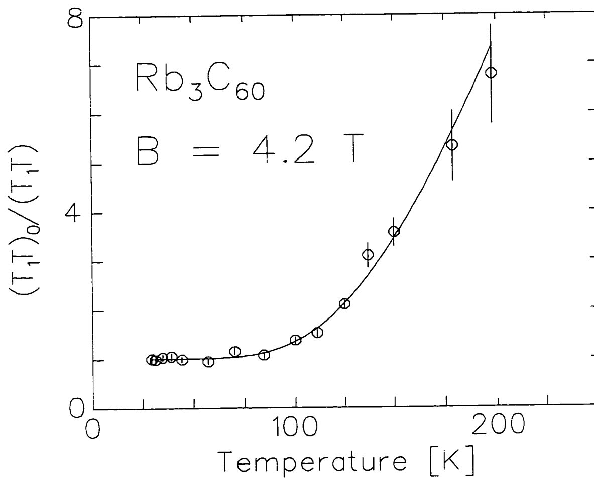
Figure 4.16: Activated increase in (T_1T)^{-1} relative to its value at low temperature likely due to \text{Mu}^{\oplus}\text{C}_{60} ionizing to endohedral \text{Mu}^- . The fit curve is (1.01(3) + 123(35) \exp(-588(40)K/T)) .
