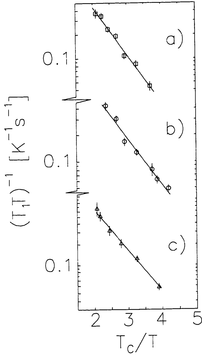
Figure 4.26: The temperature dependence of (T_1 T)^{-1} at 0.3T at low reduced temperature. a) and b) two samples of \text{Rb}_3\text{C}_{60} , and c) \text{K}_3\text{C}_{60} . This behaviour corresponds to the region labelled "Arr" in Fig. 3.12.
