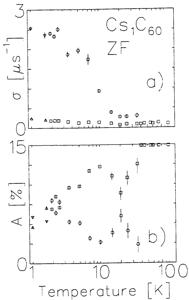
Figure 6.38: Temperature dependence of the zero field relaxation in \text{Cs}_1\text{C}_{60} . The fit function is the sum of 2 Gaussian relaxations. a) The fast and slow Gaussian relaxation rates and b) The amplitudes of the fast and slow signals. The triangles and nablas are from data taken at a different time on the same sample in a different spectrometer.
