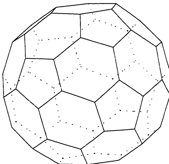
Figure 1.1: A truncated icosahedron: The geometric form has 60 vertices, 12 pentagonal faces, and 20 hexagonal faces. The C_{60} molecule contains a carbon at each vertex, C-C double bonds along the lines separating hexagons, C-C single bonds along the hexagon-pentagon boundaries, and has a diameter of roughly 7.1Å.
