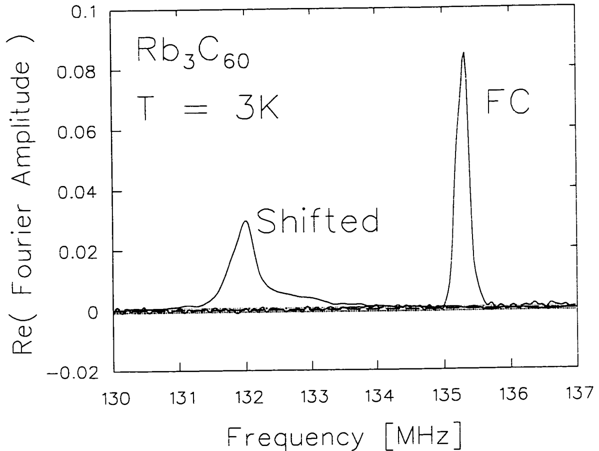
Figure 4.20: Comparison of the field-cooled (FC) lineshape with the shifted lineshape. The FC shape is the same as that shown in Fig. 4.18a. Immediately after the FC data was taken. The field was shifted down from 1T by about 0.025T at 3K in order to obtain the shifted data. The effect of shifting the field at low temperature indicates that the flux at this field is pinned (since the line broadens, unlike a vortex liquid) but not very strongly (since it shifts, unlike the case of single crystal YBCO [194]). The resemblance of the shifted lineshape to a lower \lambda vortex lattice lineshape (e.g. Fig. 4.18b) is purely coincidental. The shifted lineshape is dominated by disorder effects from the non-equilibrium field distribution.
