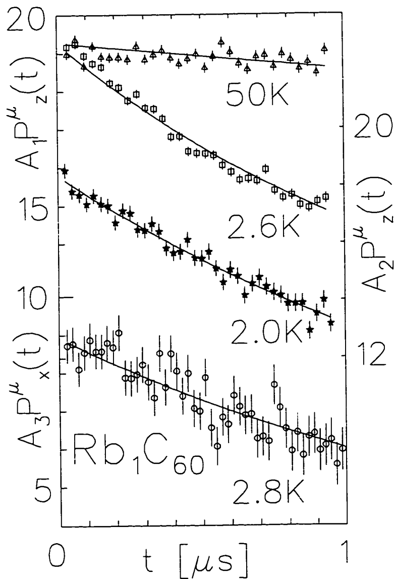
Figure 6.36: The fast component of the low temperature ZF spectrum in Rb_1C_{60} . The relaxation is well described by an exponential to the earliest accessible times. The stars correspond to data taken on a different sample. The lower data is the relaxation envelope of the decay of the TF precession at 1.5T.
