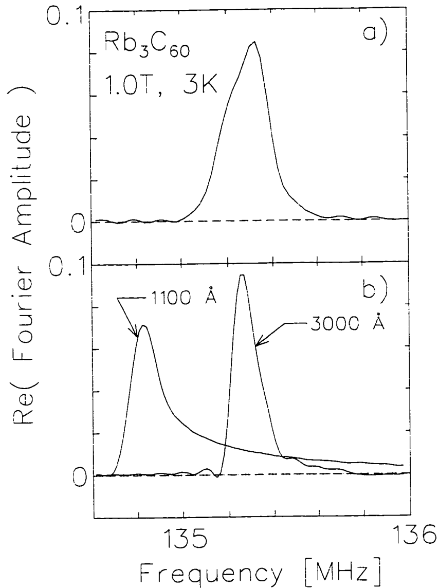
Figure 4.18: a ) A high statistics \mu SR lineshape (FFT of TF asymmetry spectrum) in Rb_3C_{60} field-cooled to 3K at 1.0T applied transverse field. b ) Simulated lineshapes for a perfectly ordered triangular flux-lattice using the Ginzburg-Landau theory.[191, 192, 193] The simulation parameters (\lambda, \xi) are (3000\text{\AA}, 30\text{\AA}) and (1100\text{\AA}, 30\text{\AA}) . The field distributions are convoluted with a Gaussian corresponding to the normal state linewidth. The 3000Å simulation also includes a small non-relaxing background signal known to exist in the data.
