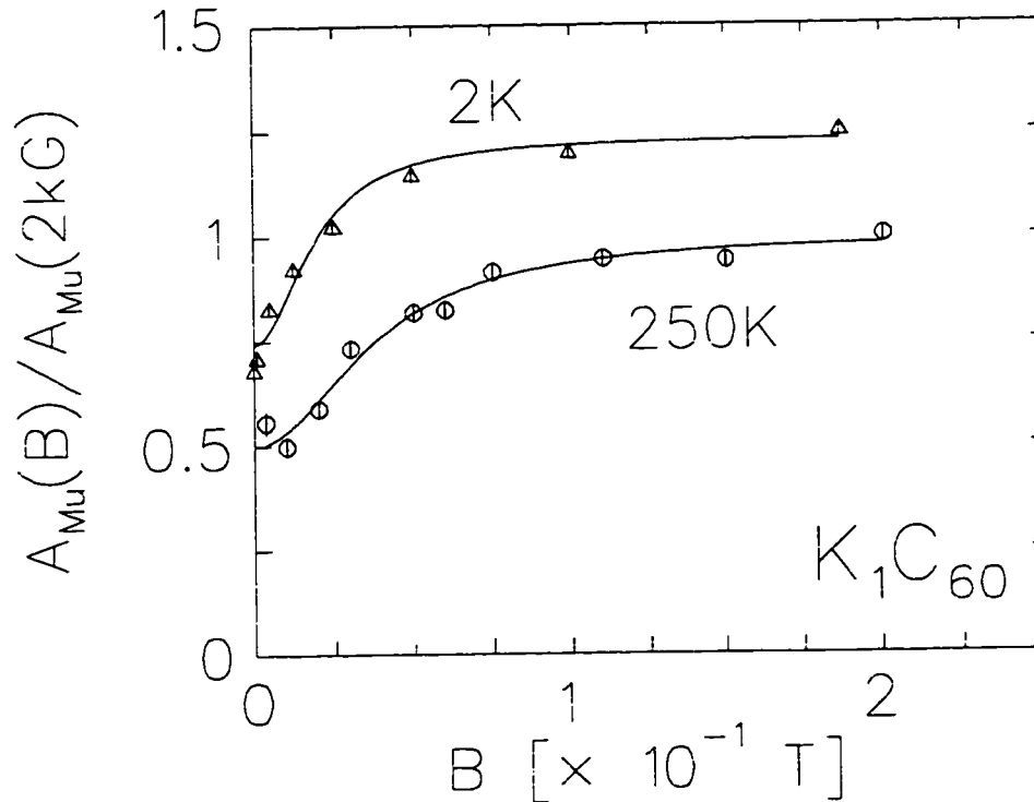
Figure 6.46: Decoupling curves of Mu in \text{K}_1\text{C}_{60} at 2K and 250K. The fits are to Eq. (4.4), and they yield isotropic hyperfine parameters of 500(100)MHz and 1070(100)MHz respectively. This behaviour is in contrast to that in \text{Rb}_3\text{C}_{60} (Fig. 4.15). The 2K curve is shifted up by 0.25 for clarity.
