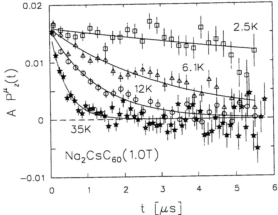
Figure 4.22: Single exponential relaxation of \text{Mu@C}_{60} in a longitudinal applied field of 1.0 T. The fits shown are to a common amplitude exponential relaxation.
