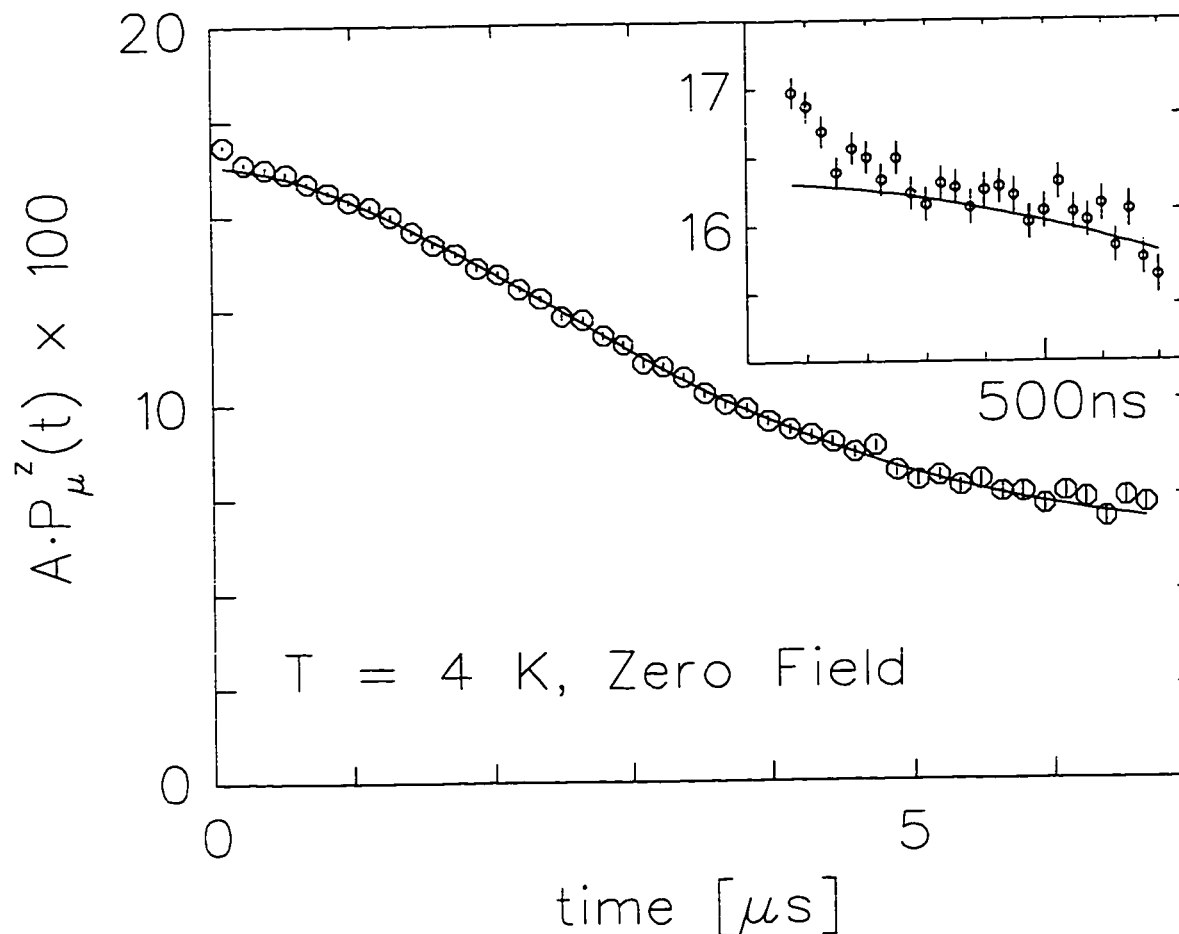
Figure 4.28: A high statistics zero applied field time spectrum in the Meissner state of \text{Rb}_3\text{C}_{60} at 4K. The slow gaussian relaxation is attributed to the diamagnetic interstitial muons relaxing in the distribution of magnetic fields of the randomly oriented static nuclear dipoles, while the small fast relaxing component (inset) is probably due to relaxation of the endohedral \text{Mu}@\text{C}_{60} . Both dynamic and static random magnetic fields can contribute to this relaxation. Dynamic fields could be due to remnant states within the gap as seen in finite low temperature zero bias conductance in several tunneling experiments. Static fields could be due to nearby nuclear dipoles.
