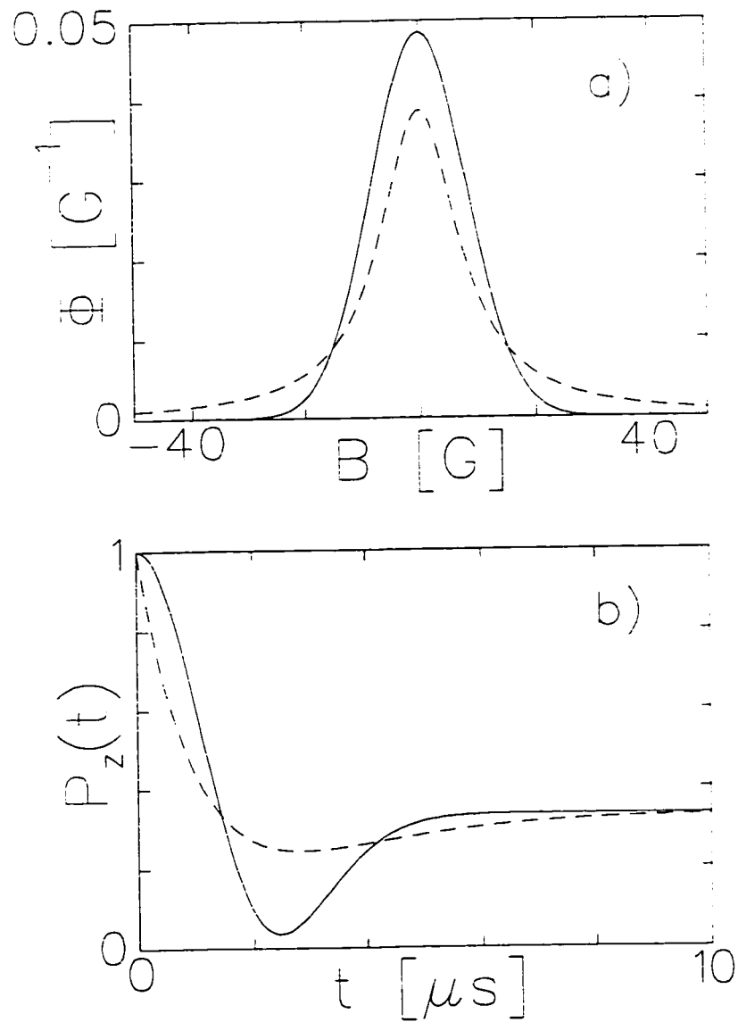
Figure 5.32: a) Gaussian (solid) and Lorentzian (dashed) field distributions and b) the corresponding Gaussian and Lorentzian Kubo–Toyabe functions for \sigma = \omega = 0.7 \mu\text{s}/2\pi\gamma_\mu .
