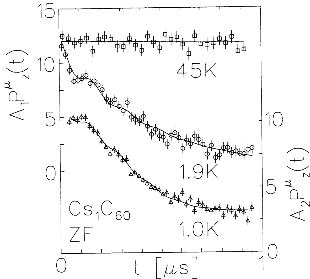
Figure 6.37: The fast component of the ZF relaxation in Cs_1C_{60} at the lowest temperature. There is a fast relaxing oscillation with a frequency of about 6MHz. The 45K data above the magnetic transition indicates that the fast component is not due to contamination from the early time straight through peak which does not occur in the sample spectra of the separate spectra apparatus.
