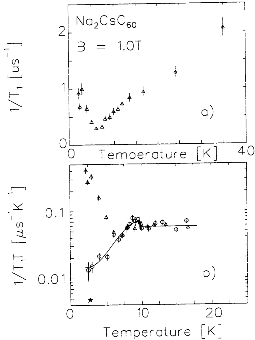
Figure 4.30: Quench rate dependence of the \text{Mu}@C_{60} T_1 relaxation rate in \text{Na}_2\text{CsC}_{60} . All data are from the same sample. triangles : non-superconducting run, circles : superconducting run, stars : fast quench. Note that above about 10K, the values of T_1T in both runs are about the same. The line is the same fit as in Fig. 4.31a.
