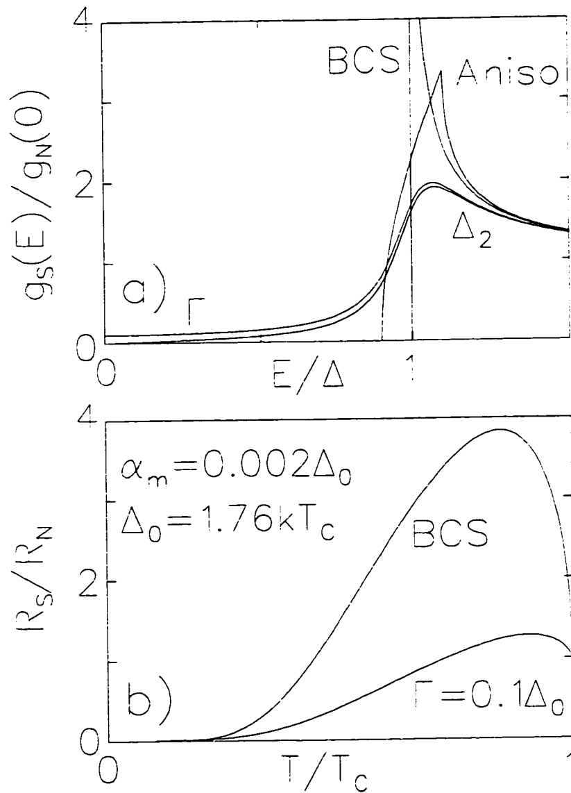
Figure 3.11: a) Models of the superconducting DOS: BCS is g_S of Eq. (3.8). Aniso is g_A (Eq. (3.11)) with a gate function distribution P(a) of width 0.1\Delta . \Gamma is g_D (Eq. (3.12)) with \Gamma = 0.1\Delta , and \Delta_2 is g_{SC} (Eq. (3.13)) with \Delta_2 = 0.1\Delta . b) The value of the Hebel-Slichter integral for the BCS and lifetime (Eq. (3.12)) broadened g_S(E) . The magnetic inelasticity parameter ( \alpha_m ) is appropriate for \text{Mu@C}_{60} in \text{Rb}_3\text{C}_{60} . The BCS temperature dependence \Delta(T) was used.
