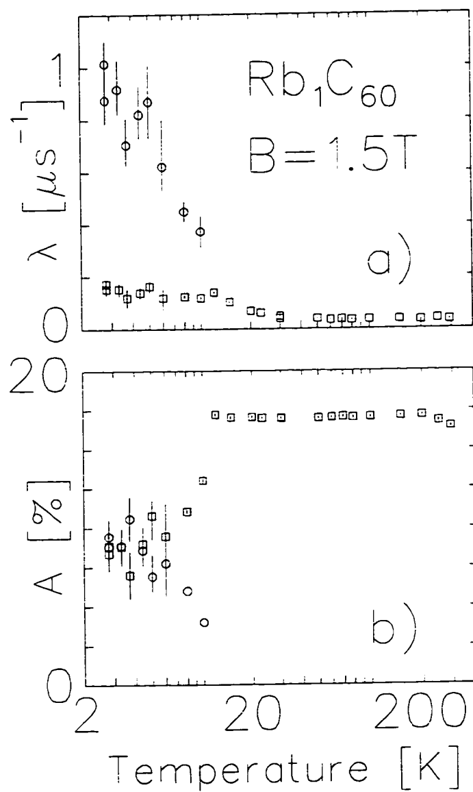
Figure 6.41: The a) exponential relaxation rates and b) corresponding amplitudes of the two relaxing signals from fits to the 1.5T TF relaxation. The third (non-relaxing) component was held fixed with temperature. Note the saturation to equal amplitudes of the two components.
