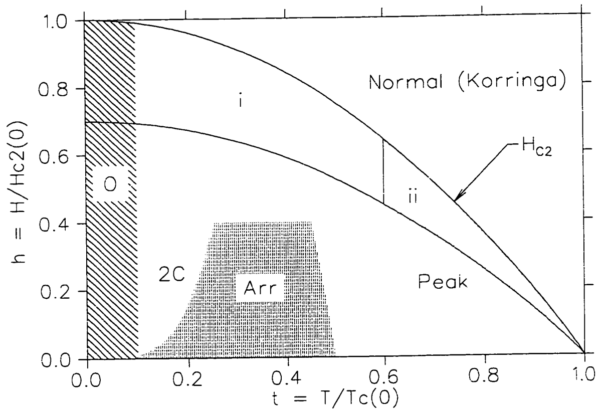
Figure 3.12: A generic phase diagram for the behaviour of (T_1T)^{-1} in a conventional type-II superconductor as described in the text.
