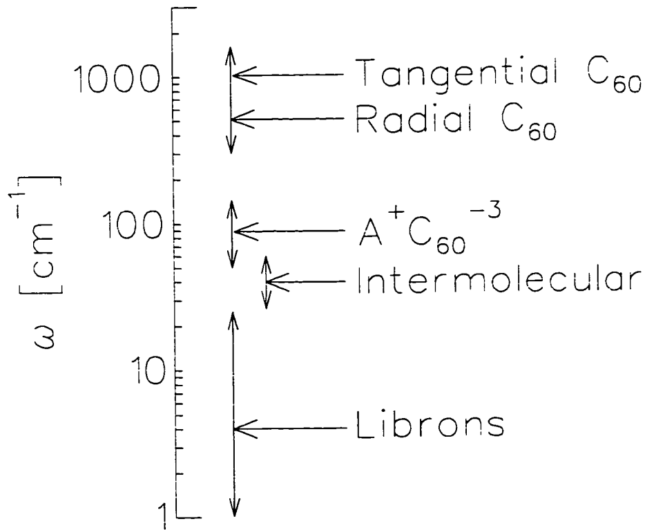
Figure 1.4: The range of phonon frequencies in A_3C_{60} with their characterizations. The high frequency range is characteristic of C_{60} molecular vibrations. The intermolecular modes, including those characteristic of vibrations of the ionic alkali fulleride bond exist at intermediate ranges. At low frequency, there are C_{60} rotational modes, i.e. librons.
