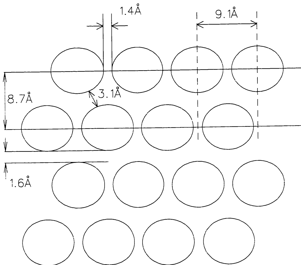
Figure 1.5: The C_{60} chains in \sigma\text{-A}_1C_{60} shown in a plane which includes the nearest neighbour chains. The distances are for A = Rb , and come from the results reported in [59].
